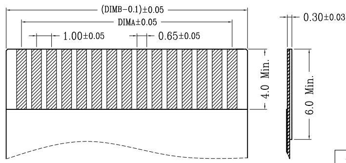
适用扁平线 (Applicable Flat Cable)
