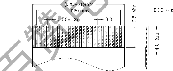
适用扁平线 (Applicable Flat Cable)
